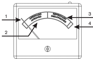
Figure 3 - Galvanometer panel
